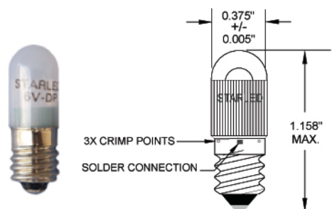
MODEL: MS1131
