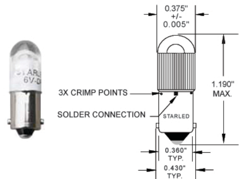
MODEL: MB1131
