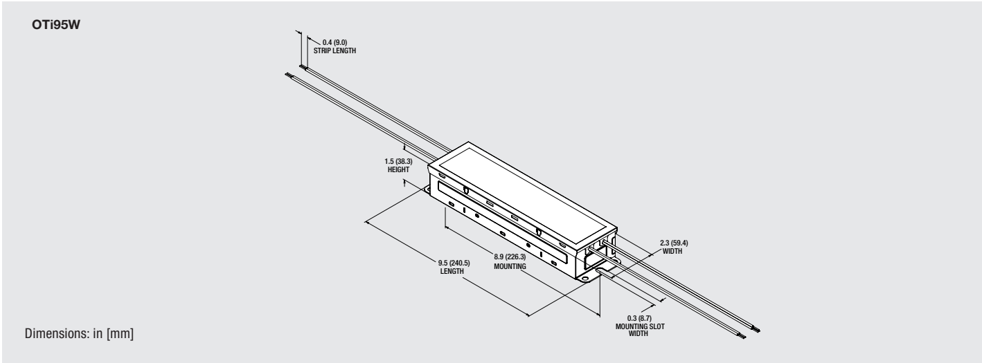
Wiring Diagram for OTi95W
