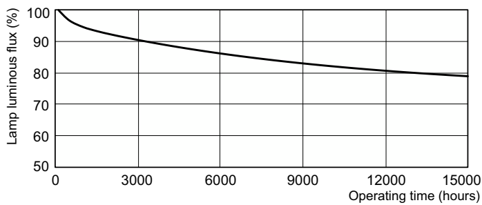
Lumen Maintenance Diagram - PL-T 32W/830/A/4P 1CT/5X10BOX ALTO
