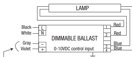
QUICKTRONIC 1x54PHO-DIM
