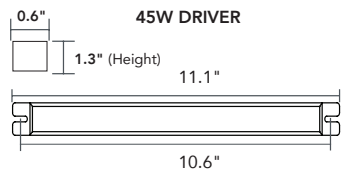
45W DRIVER
