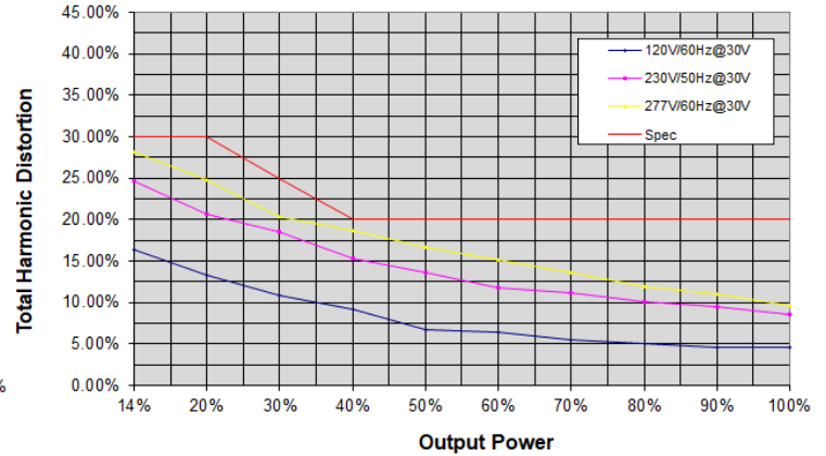
THD vs. Output Power
