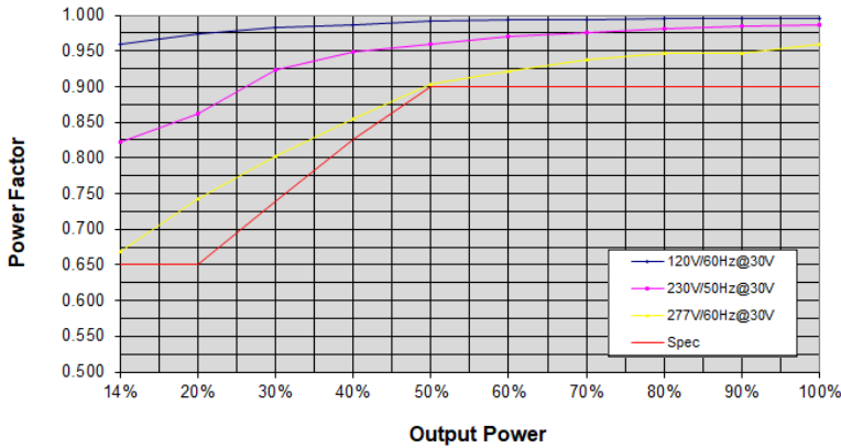
PF vs. Output Power
