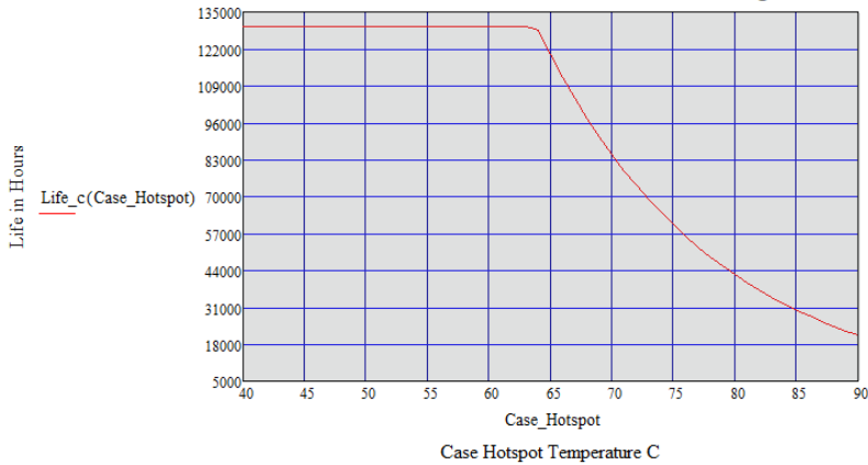
SLED 240W-XX-PCXXXX-RD Estimated Life Full Load @ 120Vac
