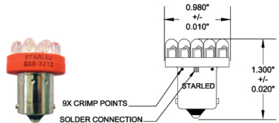
MODEL: SSB-320X-0X
