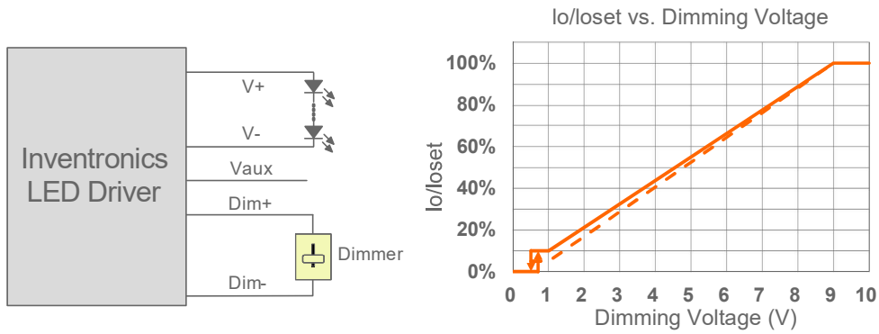
Implementation 1: Positive logic
