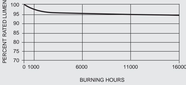
Lamp Lumen Maintenance
