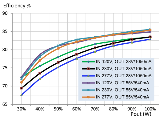
Typical Efficiency vs. Pout at 25°C Ambient Temp
