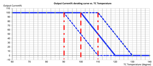
Output Current Derating vs. TC Temperature Curve
