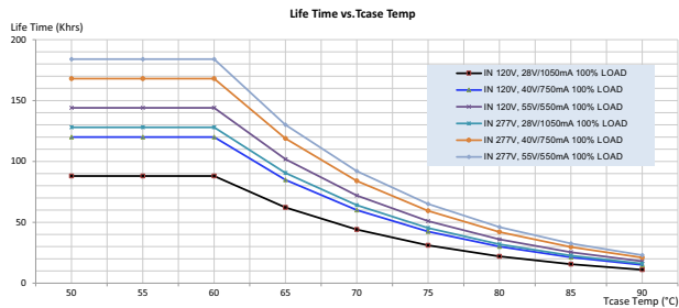
Life Time vs. Tcase Temp
