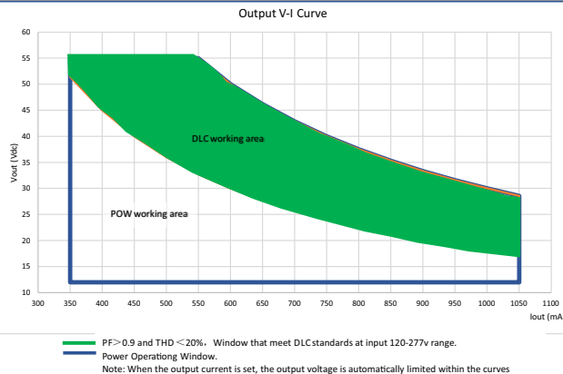
Power Operating Window & DLC Window
