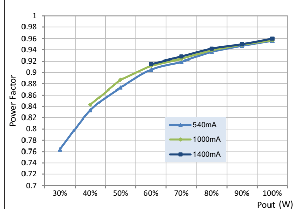
Power Factor vs Output Voltage at 277Vac
