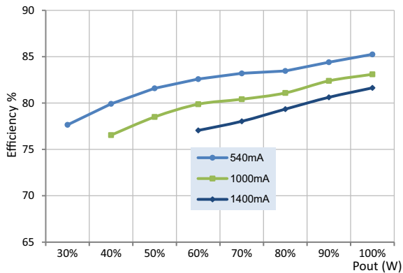
Efficiency vs Output Voltage at 277Vac
