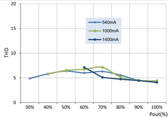
THD vs Output Voltage at 120Vac
