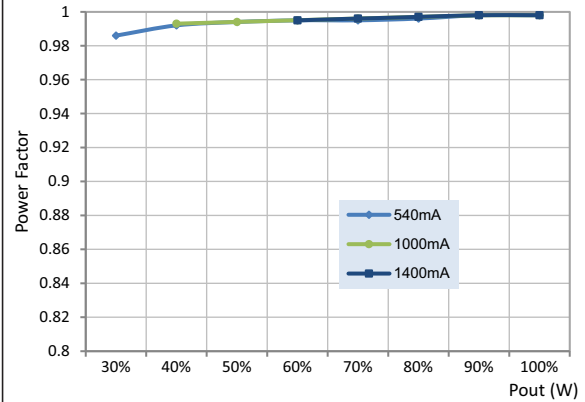
Power Factor vs Output Voltage at 120Vac
