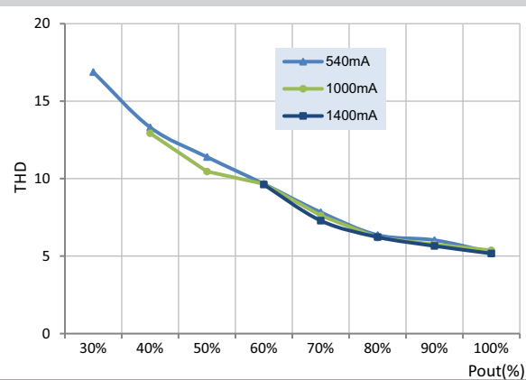
THD vs Output Voltage at 277Vac
