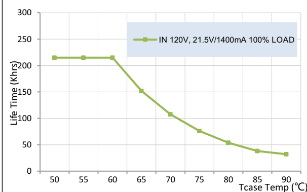
Life Time vs. Tcase Temp
