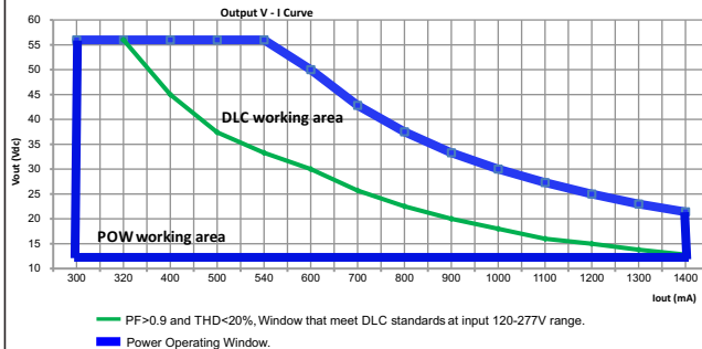
Power Operating Window & DLC Window
